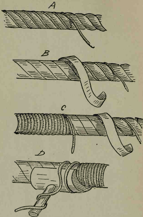
FIG. 138.—Worming, parcelling, and serving.
